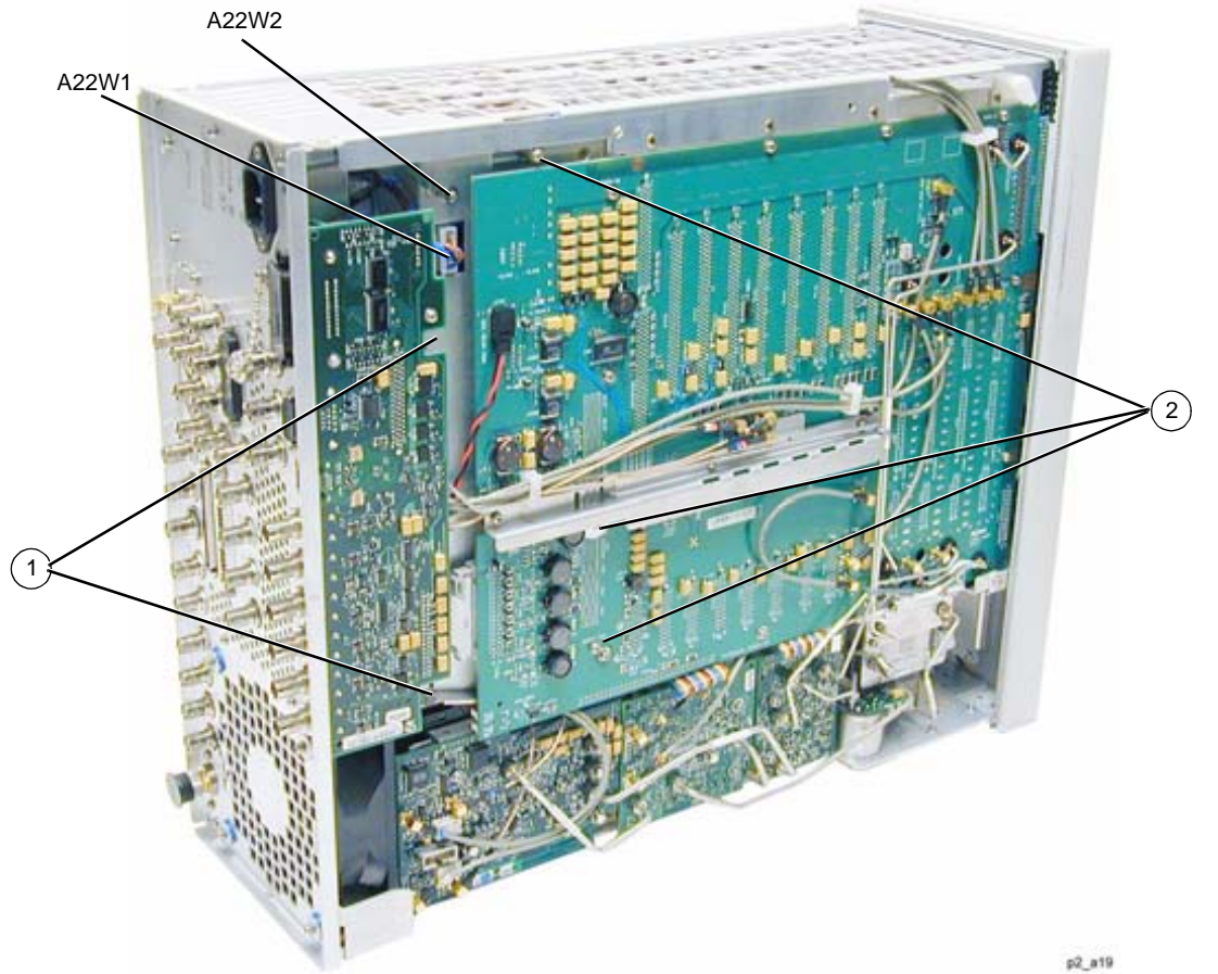
Figure 2-19 A19 Power Supply Removal
