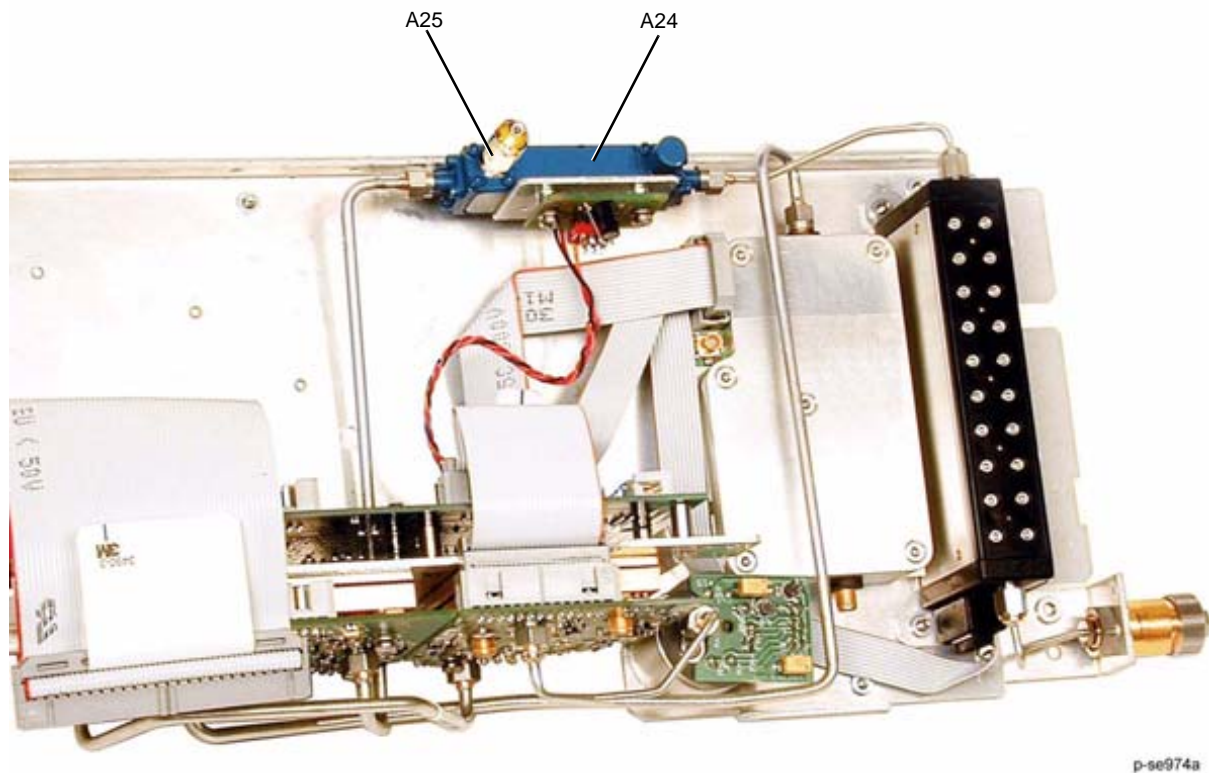
Figure 2-33 A25 40 GHz Highband Detector (Option 540)
