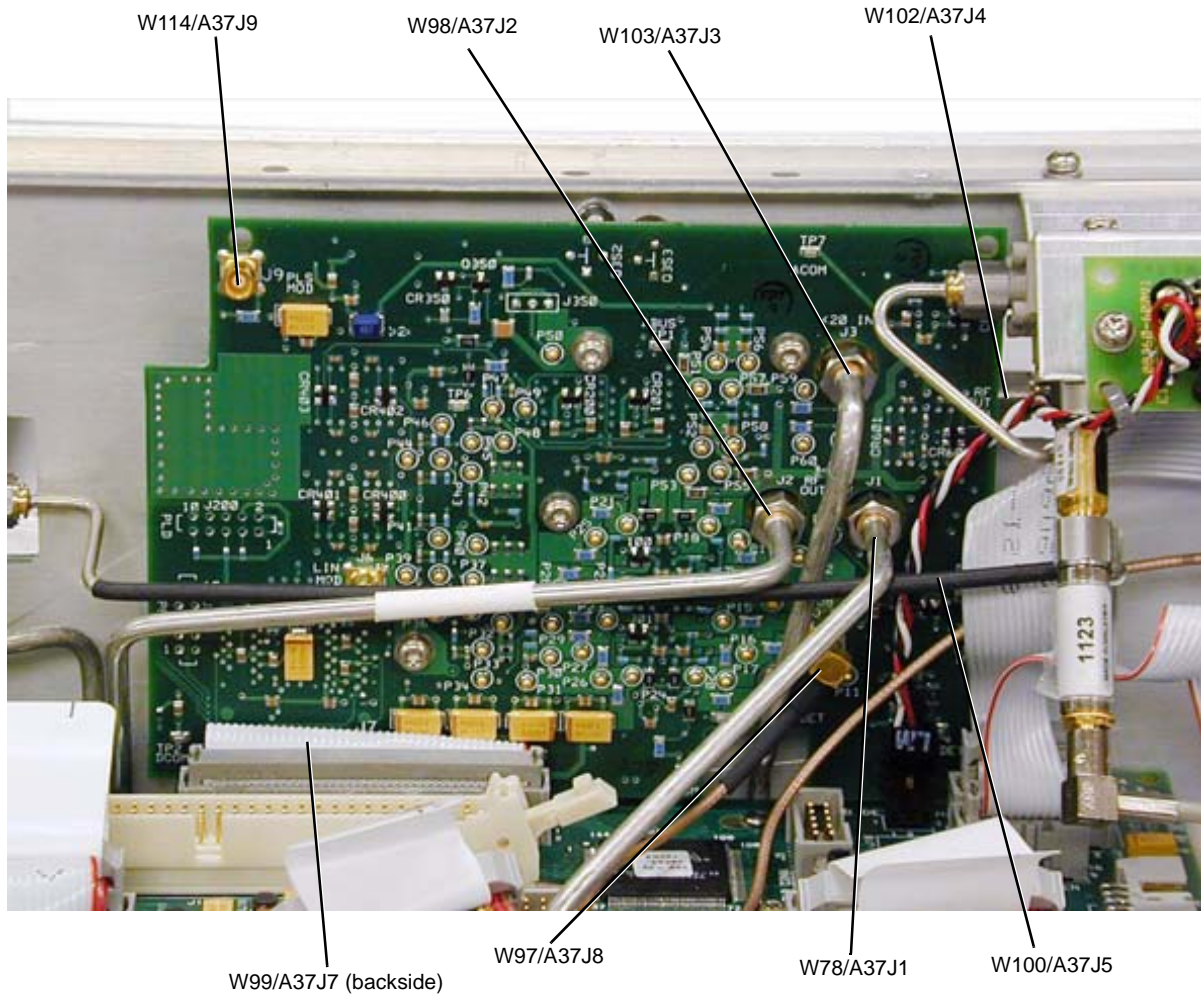
Figure 2-54 A37 Upconverter
