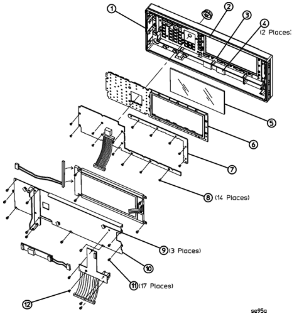
Figure 3-17 Disassembled Front Panel View
