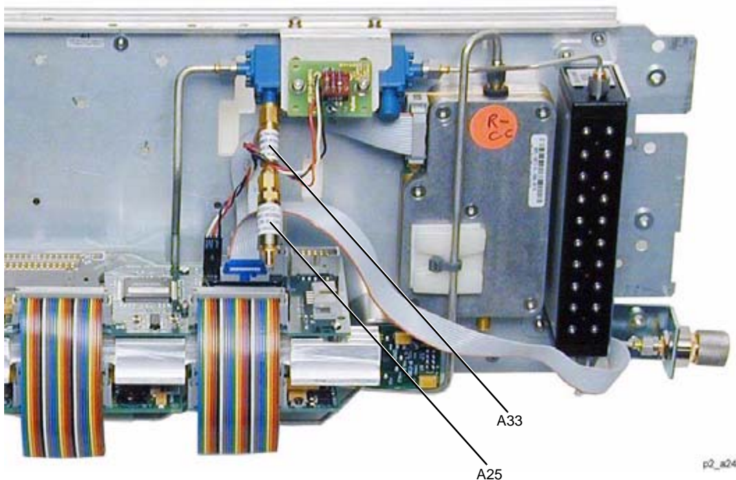
Figure 2-32 A25 20 GHz Highband Detector (Option 520)
